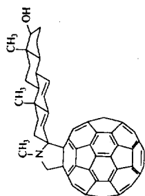
200 MHz 1 H NMR of 7
